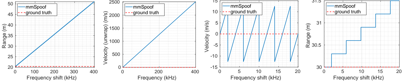
(a) Distance estimated on radar (b) Unwrapped velocity estimated on radar (c) Estimated velocity on the radar(Subset) (d) Estimated distance on the radar(Subset) Figure 5: Shows the effect of frequency shift at the mmSpoofer’s reflect array on (a) distance spoofing and (b) velocity spoofing. In particular, (c) shows a subset of estimated velocity on the radar, which illustrates the periodicity in velocity over time with a linear increase of frequency shift on reflection. (d) shows a subset of estimated distance on the radar with frequency shift, which varies in steps of \frac{1}{T_{\text{chirp}}} frequency.
